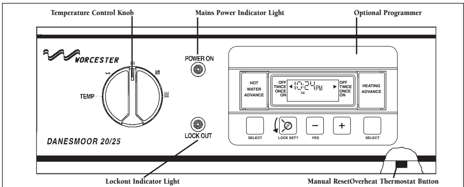
Fig. 1. Control Facia
