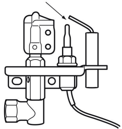
Figure 7. Pilot ignition system.
