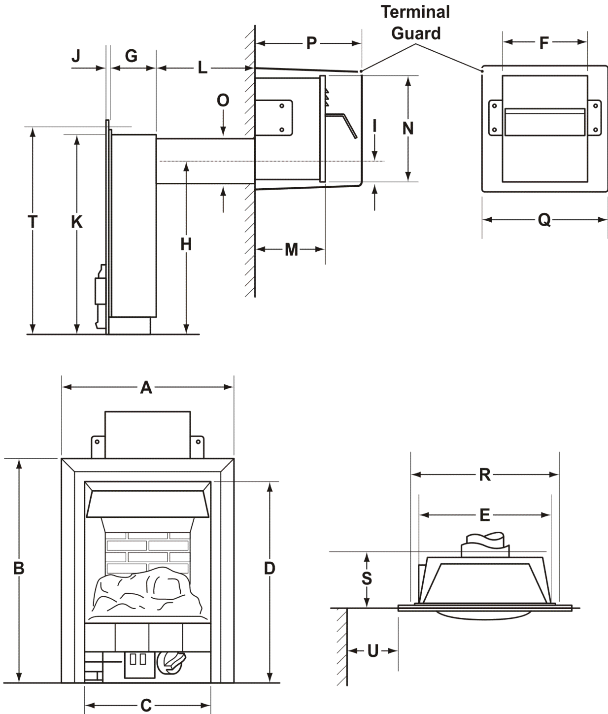
Figure 5. Appliance dimensions (Shown with fascia that is close fitted to the outer flanges of the hotbox. Dimensions 'A' and 'B' may differ depending upon the fascia fitted)
