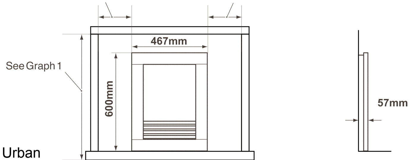
Figure 1. Appliance dimensions
