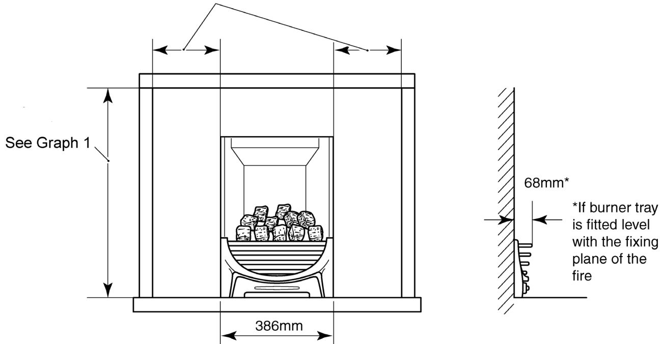
Figure 1. Appliance dimensions.
