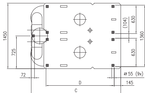
Shows the boiler's support area including the position of the support pads (shaded boxes) supplied.
