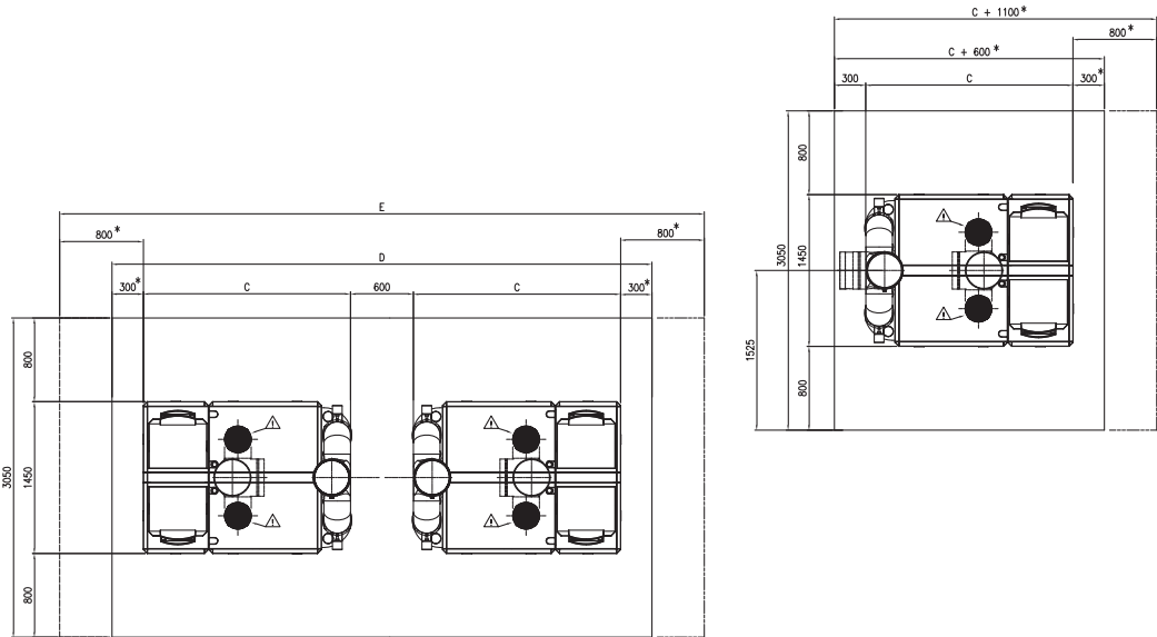
Layout in the boiler room
