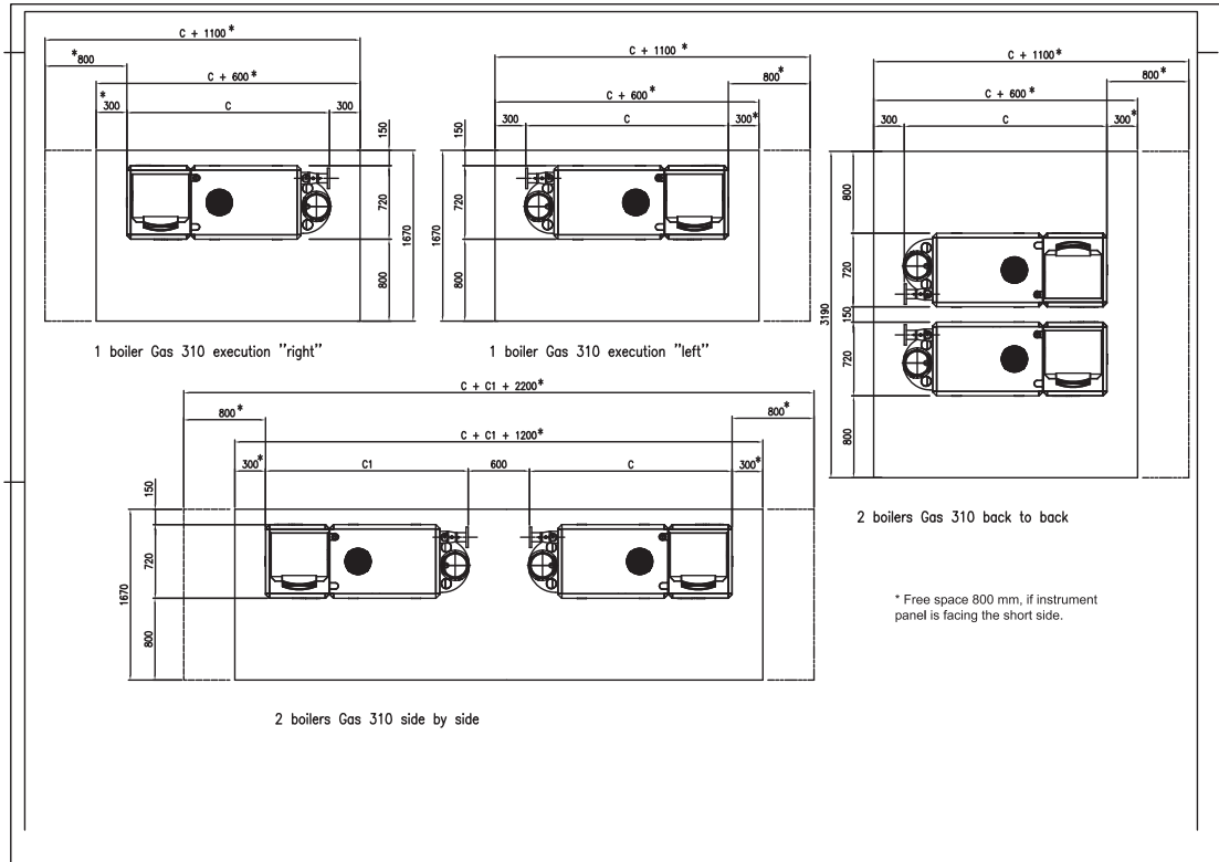
Layout in the boiler room
